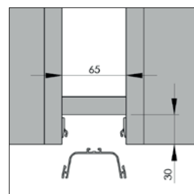
DUP65 VERTICAL
